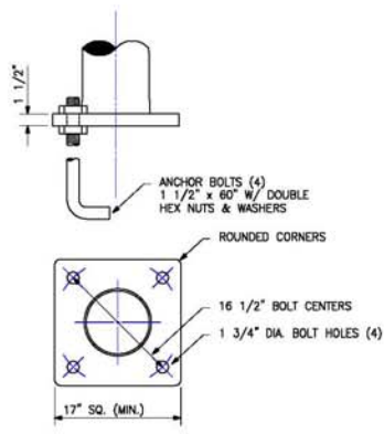
BASE PLATE DETAIL NTS
