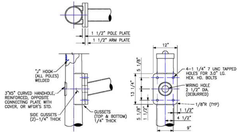
ATTACHMENT DETAIL Typical All Arm & Pole Plates charted this sheet NTS
